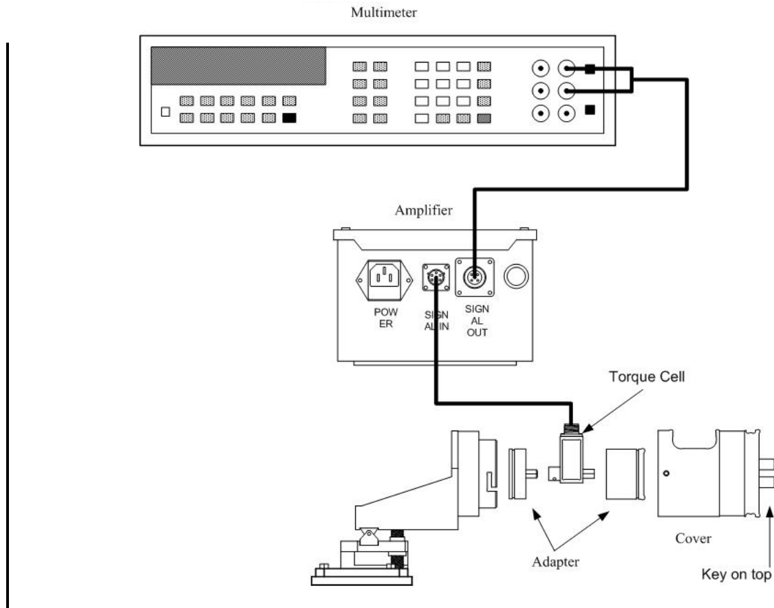
Figure 1. Electrical connection configuration.
